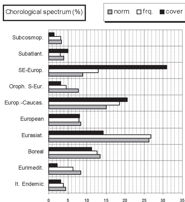
Figure 4: Chorological spectrum of Listero-Quercetum cerridis .
